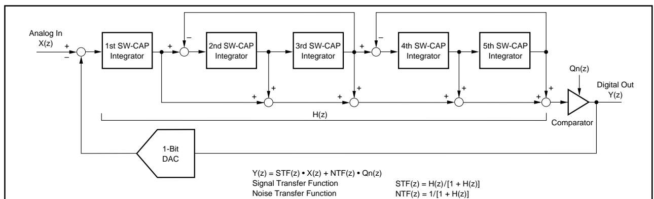
FIGURE 14. Simplified 5th-Order Delta-Sigma Modulator.
