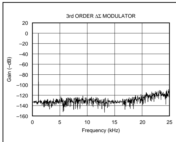
FIGURE 16. Quantization Noise Spectrum.
